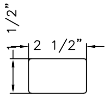
END VIEW OF RPL SLAT REPROCESSED PLASTIC LUMBER FULL SIZE
