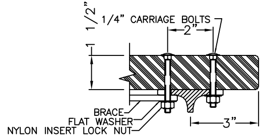
END VIEW OF RPL SLAT RECYCLED PLASTIC LUMBER
