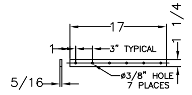
SEAT BRACE FOR RPL
