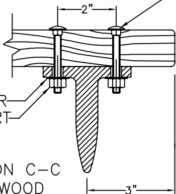
1/4" CARRIAGE BOLTS
