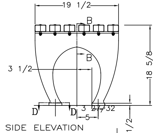
PLAN VIEW OF LEG
