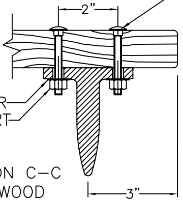
1/4" CARRIAGE BOLTS
