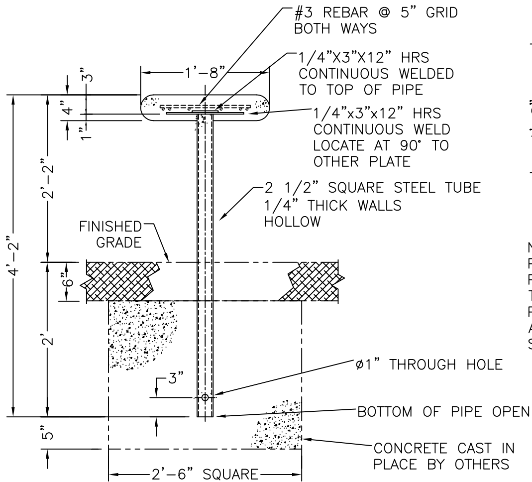
ELEVATION - FULL SECTION
