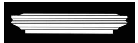
NO. 3548 ADAPTOR Cast Stone 2 3/8" h X 10 3/4" sq. base X 11" sq. top X 14 1/2" sq. at widest point
