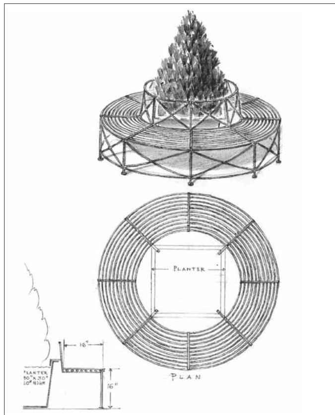
NO. 3360 ROUND THE TREE BENCH
