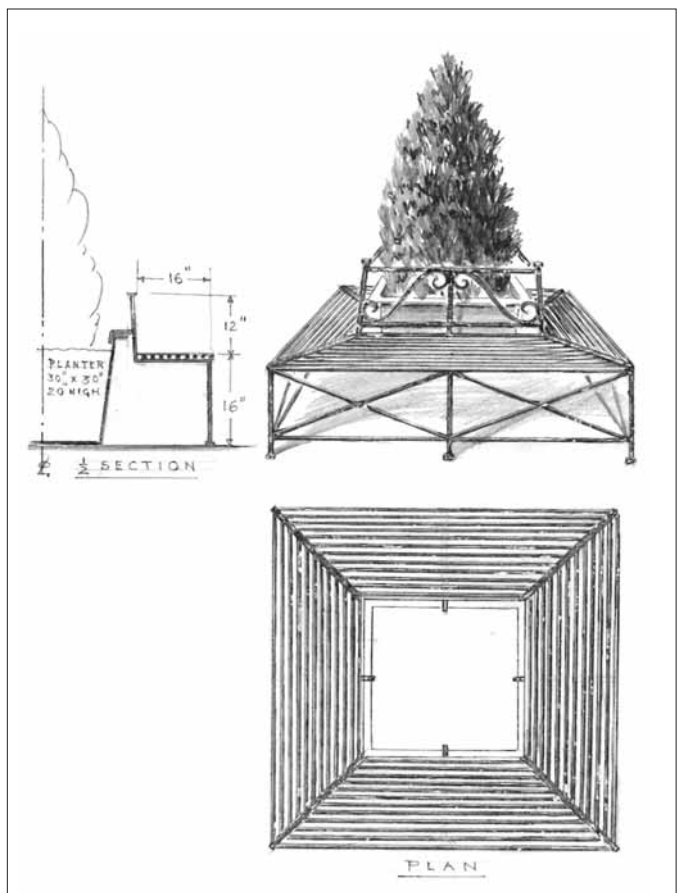
NO. 3361 ROUND THE TREE BENCH
