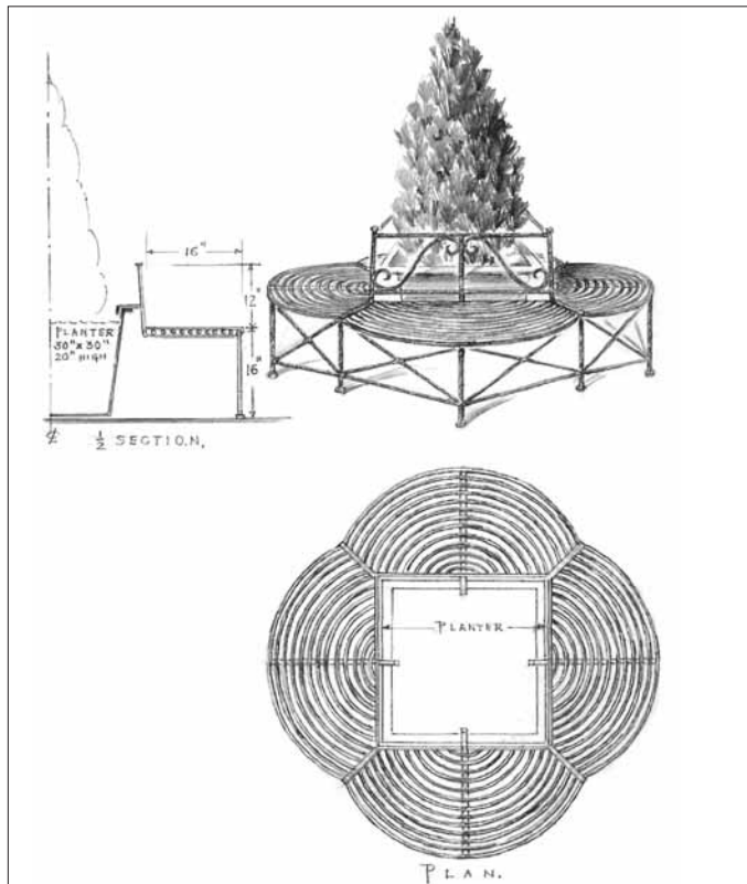
NO. 3359 ROUND THE TREE BENCH
