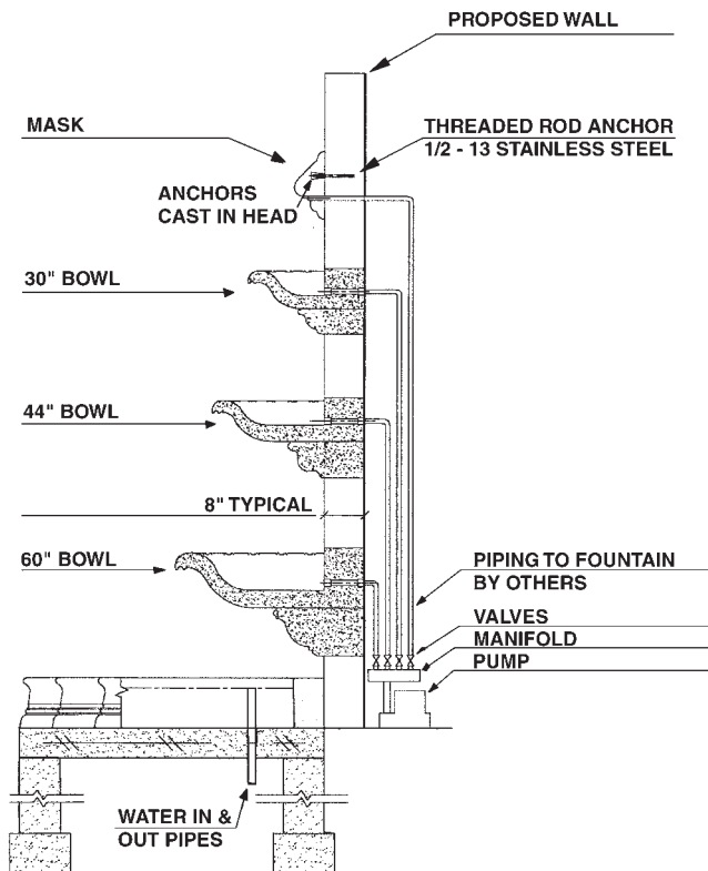
CROSS SECTION: BOWL BUILT INTO WALL THIS IS THE PREFERRED INSTALLATION
