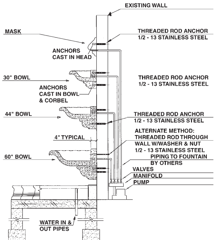
CROSS SECTION: BOWL ATTACHED TO WALL
