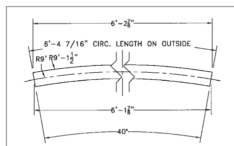
EXISTING MOLDS
