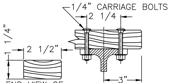
END VIEW OF WOOD SLAT IPE/BETHABARA /TABEUIA
