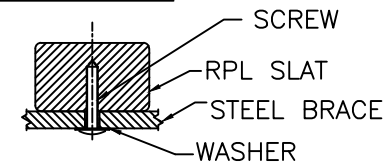
SECTION VIEW OF RPL SLAT CROSS BRACE PLACED UNDER SLAT AND OVER THE CHANNEL
