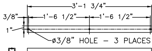
CHANNEL BRACE FOR RPL SLATS MAT'L: 3/16" x 1" x 2" STEEL CHANNEL 4 REQUIRED
