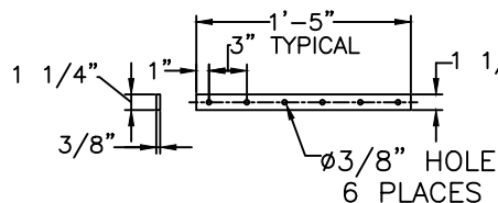
SEAT BRACE FOR RPL 3/8" X 1 1/4" X 17" LG HRS. 2 PIECES
