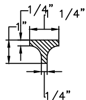
TYPICAL SECTION
