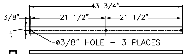
CHANNEL BRACE FOR RPL SLATS MAT'L: 3/16" x 1" x 2" STEEL CHANNEL 4 REQUIRED
