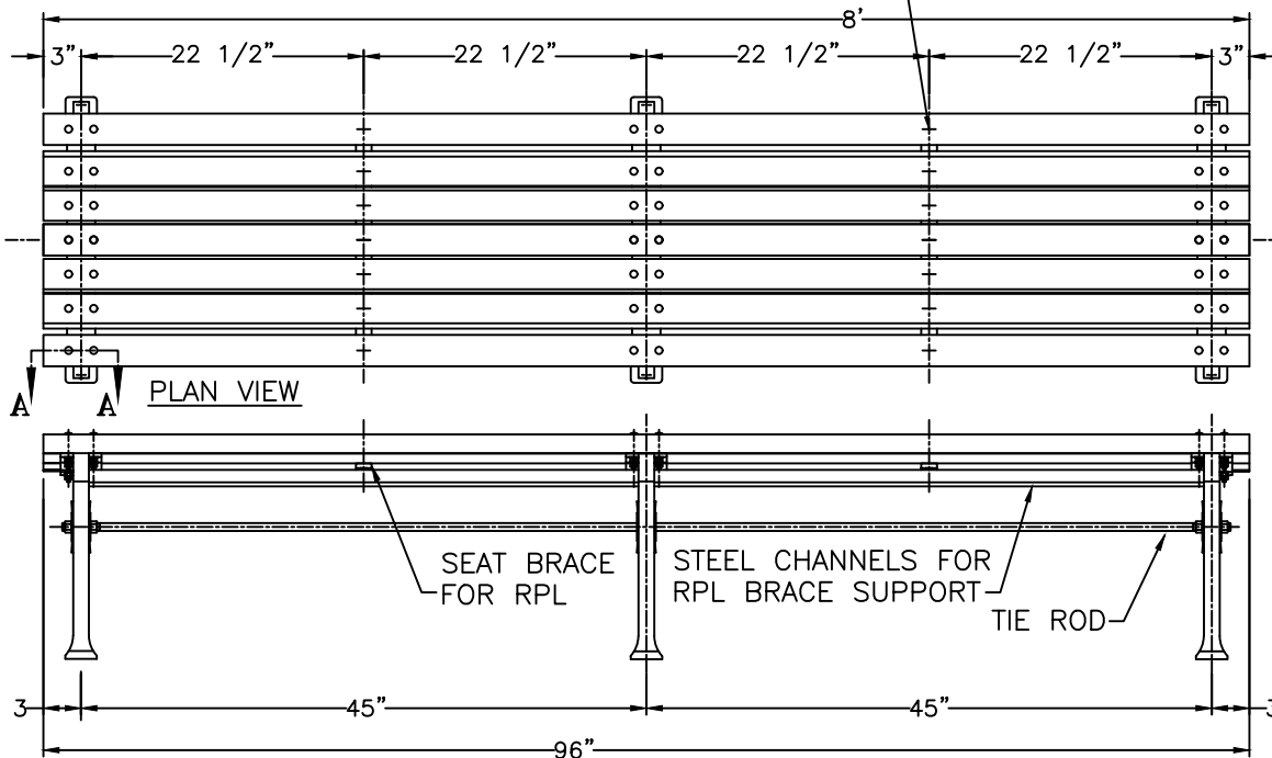
FRONT ELEVATION
